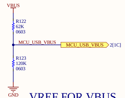
VREF FOR VBUS
