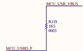
Pull-up for D +
